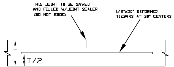
CONSTRUCTION JOINT
