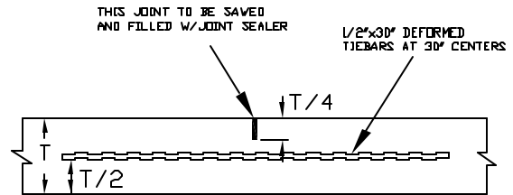
CONTRACTION JOINT
