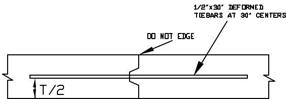
CONSTRUCTION JOINT
