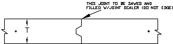
CONSTRUCTION JOINT (KEYED)
