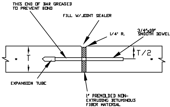
EXPANSION JOINT
