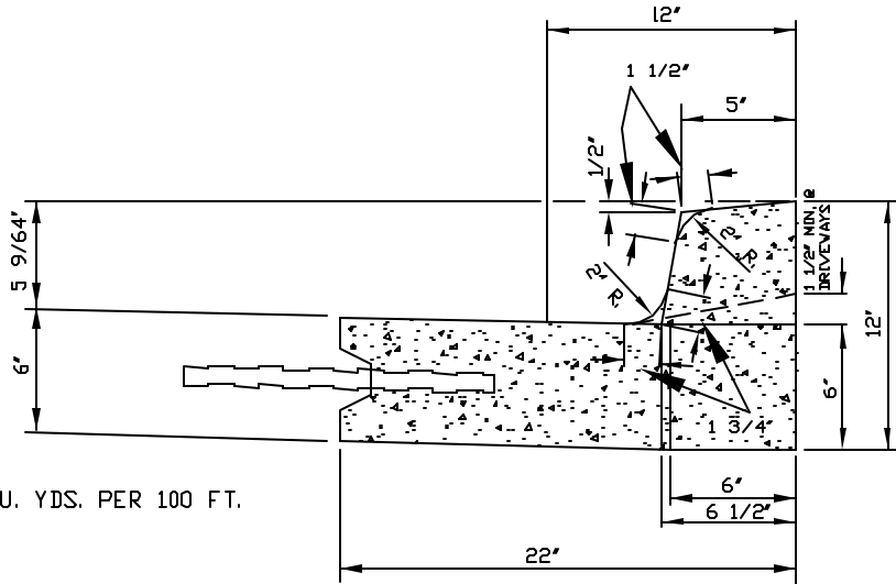
COMBINATION CONCRETE BATTERED CURB AND GUTTER
