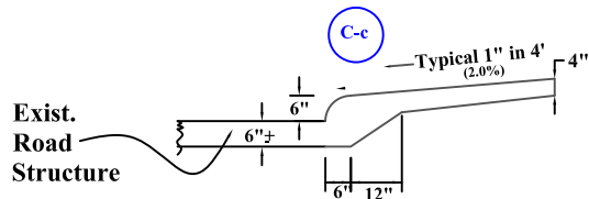
Typical Sidewalk Section
